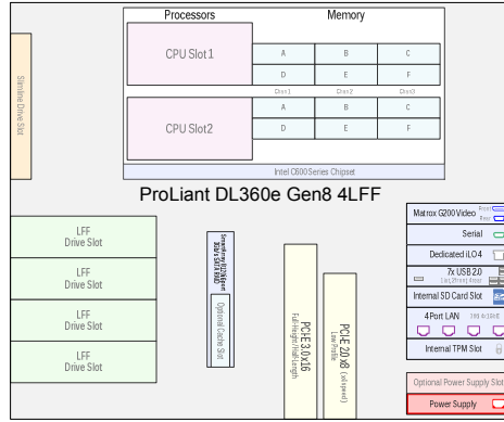
4 LFF SAS/SATA Hot Plug Drive Bays
