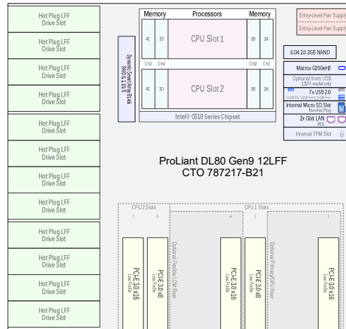
12 LFF SAS/SATA Non-hot Plug Drive Bays
