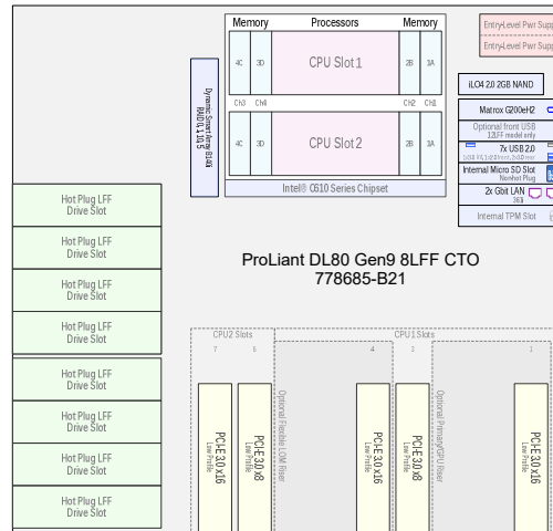
8 LFF SAS/SATA Non-hot Plug Drive Bays
